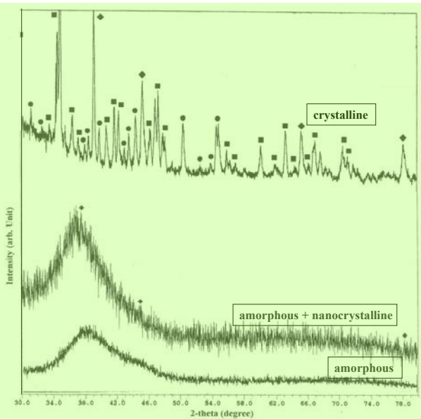
Figure 2. X-ray diffraction patterns ( \text{Cu K}\alpha radiation at 40 kV and 35 mA) for the melt-spun \text{Al}_{87}\text{Co}_{8.7}\text{Ce}_{4.3} alloy ribbon (52 m/s wheel speed) showing the amorphous microstructure of the as-quenched material, the amorphous + nanocrystalline microstructure of the 100 hour 100°C treatment, and the crystalline microstructure which is developed after a non-isothermal 550°C heat-treatment. 6
