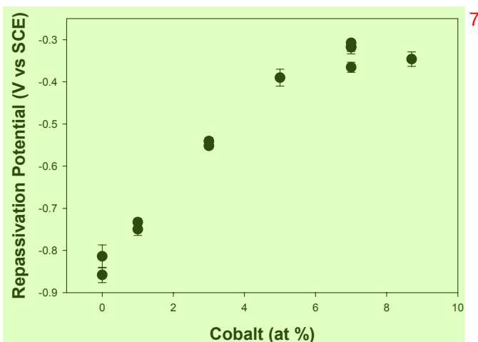
Figure 6. Repassivation potential for as-spun Al-Co-Ce alloys with 0 to 8.7 atomic percent cobalt in deaerated 0.6 M NaCl solution (pH 6) expressed as a function of cobalt. Alloys with >1% Co are fully amorphous while those with 0-1% Co contain nanocrystals.
