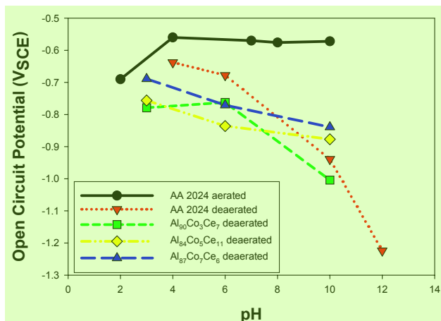
Figure 3. Open circuit potentials for amorphous Al-Co-Ce alloy and AA 2024 after one-hour exposure to 0.6 M NaCl solution with pH adjusted using 1 M HCl or 1 M NaOH as necessary.
